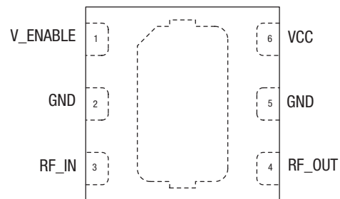
Figure 2. SKY65404-31 Pinout (Top View)
